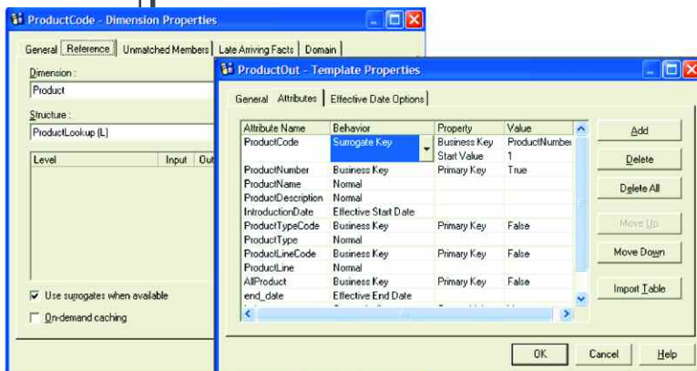
Automated surrogate key management dimensions and facts
